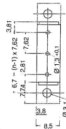
Pin layout
